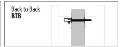
Optional Mounting
