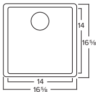
Karran Q-315 Min. Cabinet Required: 21" O.D. 16-5/8" x 16-5/8" x 8" Colors: White, Bisque, Grey, Black, Concrete, or Brown
