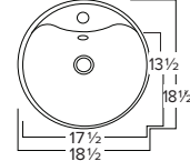
Chemcore CONE O.D. 18-1/2" x 18-1/2" x 6-1/4" Bowl Depth: 4-1/2" White
