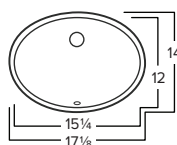
Chemcore ACORN O.D. 17-1/8" x 14" x 7-3/4" Bowl Depth: 6" White, Bisque, or Black
