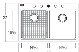
Kindred KGDL2233-9N Min. Cabinet Required: 36" O.D. 33" x 22" x 9" (Small 8") Stainless strainer basket(s) not included 1 Bottom grid included
