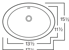
Chemcore DERBY O.D. 17-1/2" x 15-1/2" x 7" Bowl Depth: 5-1/4" White or Black
