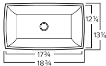
Chemcore TUB O.D. 18-3/4" x 13-1/4" x 5-1/2" Bowl Depth: 4-1/2" White or Bisque
