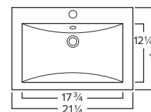
Chemcore LEDGE O.D. 21-1/4" x 18" x 6-3/4" Bowl Depth: 5" White or Bisque 1 hole or 3 hole (4" center)
