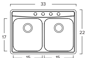
Kindred FCDLA3322-8-1CBN FCDLA3322-8-4CBN Min. Cabinet Required: 36" O.D. 33" x 22" x 8" 18 Gauge 1 or 4 Hole Strainer basket(s) not included Bottom grids available
