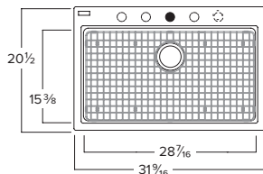
Kindred KGSL2031-8N Min. Cabinet Required: 33" O.D. 31-9/16" x 20-1/2" x 8" Stainless strainer basket(s) not included Bottom grid included
