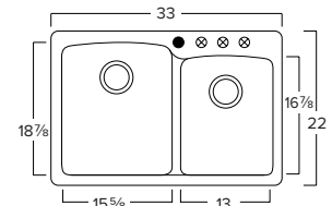
Franke EOCH33229-1 (champagne) *DWO EODB33229-1 (mocha) EOOX33229-1 (onyx) Min. Cabinet Required: 36" O.D. 33" x 22" x 9" & 8"
