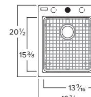
Kindred KGSL2017-8N Min. Cabinet Required: 18" O.D. 16-3/4" x 20-1/2" x 8" Stainless strainer basket(s) not included Bottom grid included
