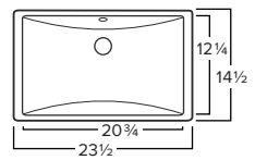
Chemcore TROUGH O.D. 23-1/2" x 14-1/2" x 7-3/4" Bowl Depth: 5-1/2" White or Bisque
