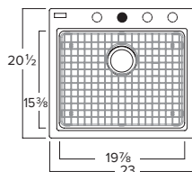
Kindred KGSL2023-8N Min. Cabinet Required: 27" O.D. 23" x 20-1/2" x 8" Stainless strainer basket(s) not included Bottom grid included
