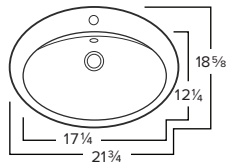
Chemcore DAISY O.D. 21-3/4" x 18-5/8" x 8-1/4" Bowl Depth: 6-3/8" White or Bisque 1 hole
