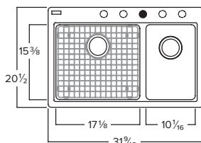
Kindred KGDC2031R-8N Min. Cabinet Required: 33" O.D. 31-9/16" x 20-1/2" x 8" (Small 7") Stainless strainer basket(s) not included 1 Bottom grid included
