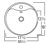
Chemcore CONE O.D. 18-1/2" x 18-1/2" x 6-1/4" Bowl Depth: 4-1/2" White
