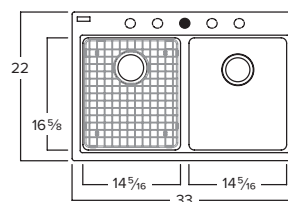
Kindred KGDL2233-9N Min. Cabinet Required: 36" O.D. 33" x 22" x 9" (Small 8") Stainless strainer basket(s) not included 1 Bottom grid included
