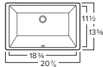
Chemcore BASIN O.D. 20-7/8" x 13-5/8" x 7-1/4" Bowl Depth: 5-1/2" White or Bisque
