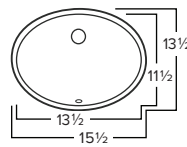
Chemcore BUD O.D. 15-1/2" x 13-1/2" x 8" Bowl Depth: 6-1/4" White or Bisque
