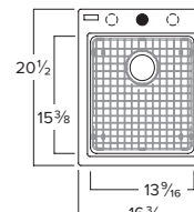
Kindred KGSL2017-8N Min. Cabinet Required: 18" O.D. 16-3/4" x 20-1/2" x 8" Stainless strainer basket(s) not included Bottom grid included
