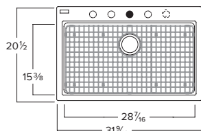
Kindred KGSL2031-8N Min. Cabinet Required: 33" O.D. 31-9/16" x 20-1/2" x 8" Stainless strainer basket(s) not included Bottom grid included
