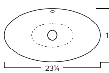
Chemcore CANOE O.D. 23-1/4" x 15" x 7-1/2" Bowl Depth: 4-3/4" White
