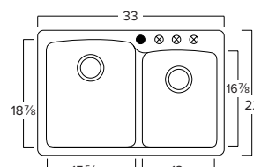
Franke EOCH33229-1 (champagne) *DWO EODB33229-1 (mocha) EOOX33229-1 (onyx) Min. Cabinet Required: 36" O.D. 33" x 22" x 9" & 8"
