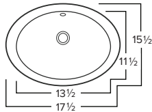
Chemcore DERBY O.D. 17-1/2" x 15-1/2" x 7" Bowl Depth: 5-1/4" White
