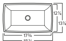
Chemcore TUB O.D. 18-3/4" x 13-1/4" x 5-1/2" Bowl Depth: 4-1/2" White or Bisque
