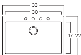
Franke DIG61091-CHA (champagne) *DWO DIG61091-MOC (mocha) DIG61091-ONY (onyx) Min. Cabinet Required: 36" O.D. 33" x 22" x 9"
