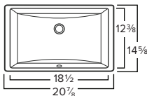
Chemcore TRENCH O.D. 20-7/8" x 14-5/8" x 8-1/4" Bowl Depth: 6-1/4" White or Bisque
