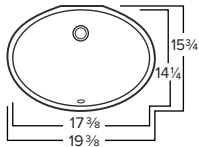
Chemcore LOTUS O.D. 19-3/8" x 15-3/4" x 8-1/4" Bowl Depth: 6-1/2" White or Bisque
