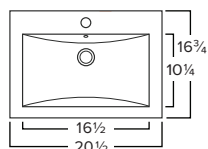
Chemcore APRON O.D. 20-1/2" x 16-3/4" x 6-7/8" Bowl Depth: 4-1/2" White or Bisque
