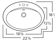
Chemcore DAISY 3-Hole O.D. 22-1/8" x 18-7/8" x 8-1/2" Bowl Depth: 6" White or Bisque 3 hole (4" center)
