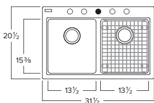
Kindred KGDL2031-8N Min. Cabinet Required: 33" O.D. 31-1/2" x 20-1/2" x 8" Stainless strainer basket(s) not included 1 Bottom grid included
