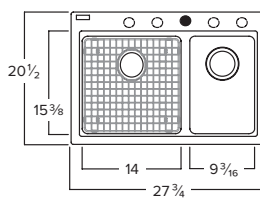
Kindred KGDC2027R-8N Min. Cabinet Required: 30" O.D. 27-3/4" x 20-1/2" x 8" (Small 7") Stainless strainer basket(s) not included 1 Bottom grid included
