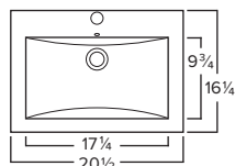
Chemcore BOX O.D. 20-1/2" x 16-1/4" x 7" Bowl Depth: 5" White or Bisque
