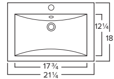
Chemcore LEDGE O.D. 21-1/4" x 18" x 6-3/4" Bowl Depth: 5" White or Bisque 1 hole or 3 hole (4" center)
